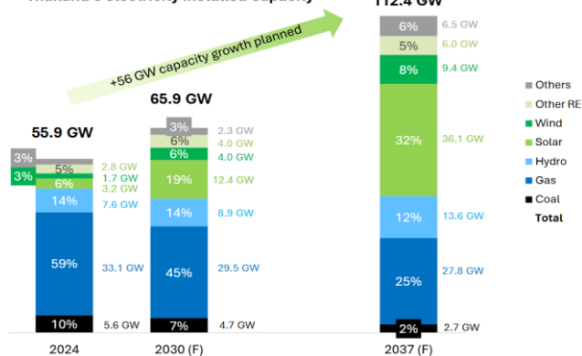
Thailand's electricity installed capacity
